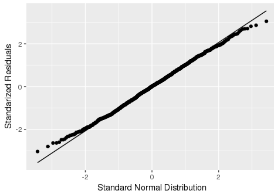
QQ Plot for Standardized Residuals
